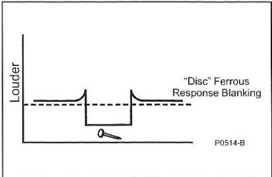
Figure 5.5 Discrimination target signal on a ferrous target.
